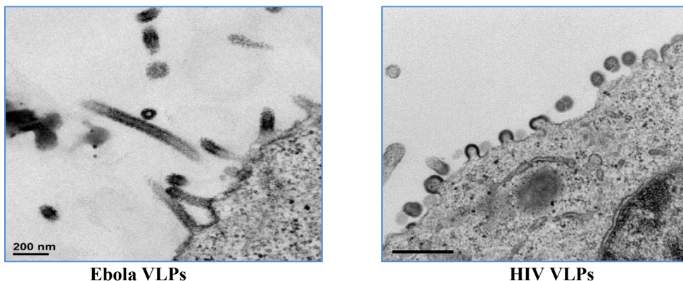
Figure 1. Electron micrographs showing the VLPs elicited by GeoVax vaccines from human cells. Note that the Ebola VLPs on the left self-assemble into the rod-like shape of the actual Ebola virus, while the HIV VLPs shown on the right take on the spherical shape of the actual HIV virus. While below the resolution of these micrographs, both types of VLPs display what we believe to be the native form of their respective viral envelope glycoproteins which we believe is key to generating an effective immune humoral response.
